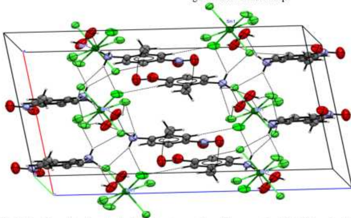
Fig-2. Packing of molecules in the structure of nonlinear optical (NLO) materials. bis(2-Methyl-4-nitroanilinium) hexachloro-Tin(IV) monohydrate
