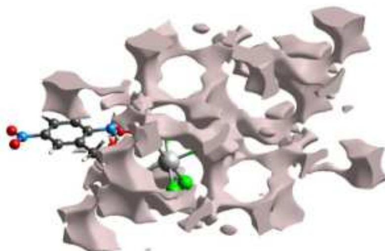
Fig-4. Crystal Voids appearance of bis(2-Methyl-4-nitroanilinium) hexachloro-Tin(IV) monohydrate.
