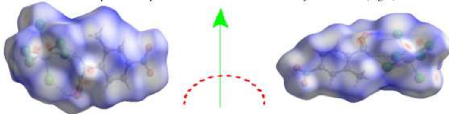
Fig-3. Hirschfeld surface of dnorma nonlinear optical (NLO) materials, interactions inside and outside the surface.
