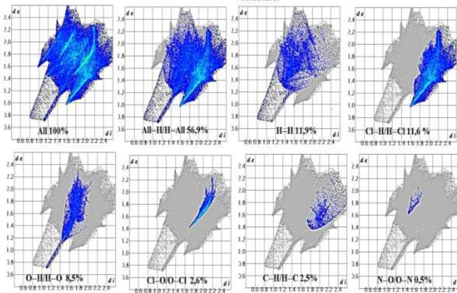
Fig-4. Fingerprint representation of a nonlinear optical (NLO) materials Hirshfeld surface, contribution of interatomic interactions to surface formation
