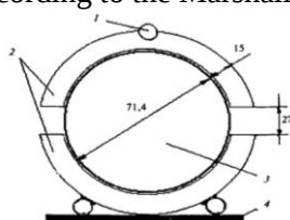
Figure 5. The process of checking the compressive strength of an asphalt concrete sample in a universal press: 1-hinge, 2-cylinder surface, 3-place for sample, 4-bottom plate.
