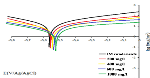
Figure-1. Polarization curves of PF-1 corrosion inhibitor at different concentrations in 1 M condensate medium for 2 hours at 298 \pm 1 K for St3 grade steel
