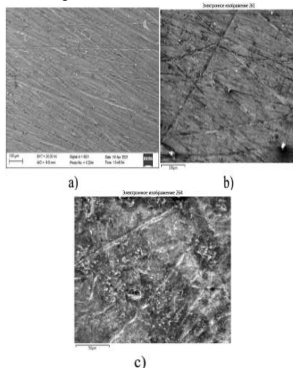
Figure-3. SEM view of ST3 steel sample a) pure metal, b) inhibitory environment, c) non-inhibitory condensate environment
