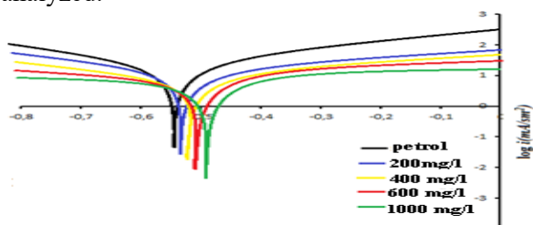
Figure-2. Polarization curves for steel grade St3 recorded for 2 hours at 298 \pm 1 K at different concentrations of corrosion inhibitor PF-1
